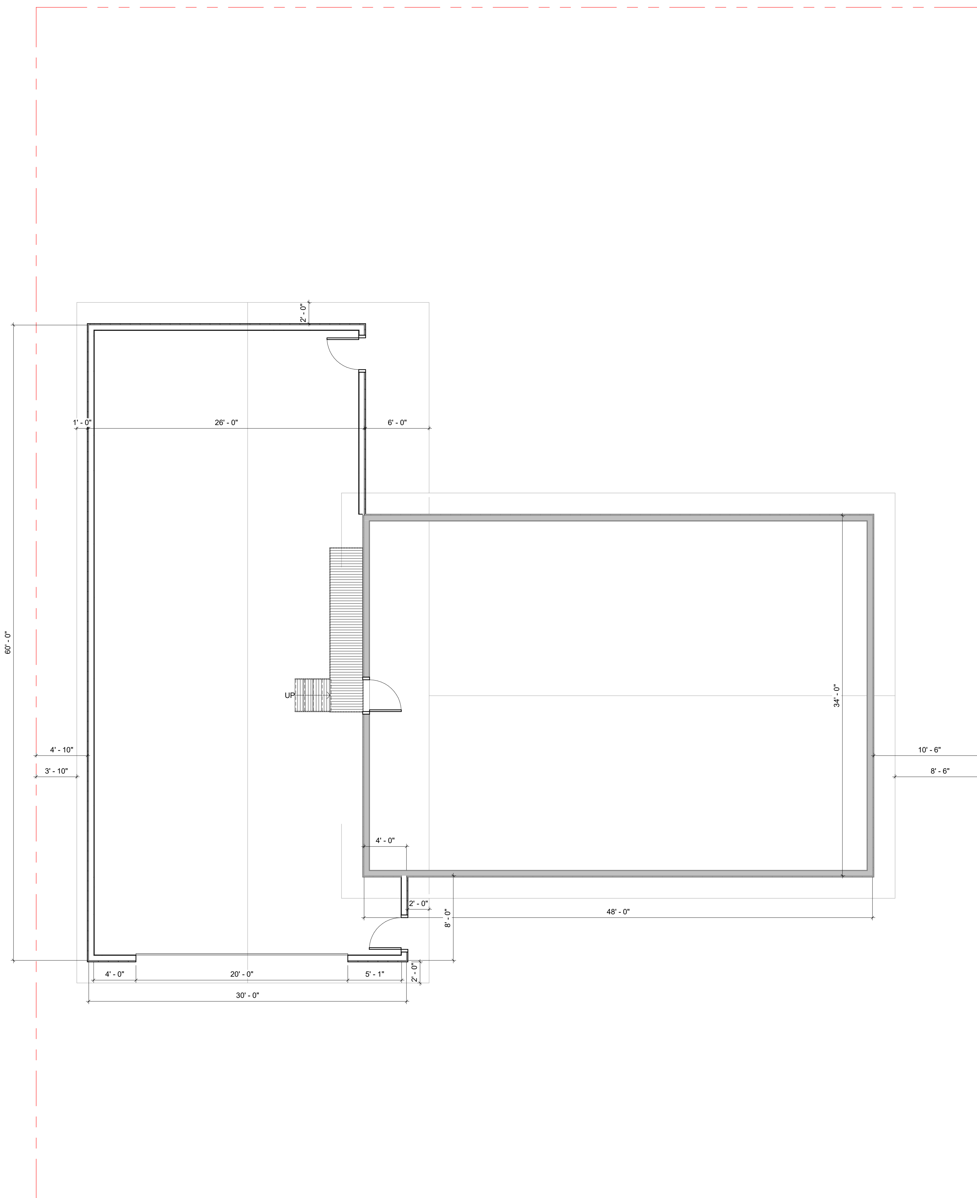
MAIN LEVEL FLOOR PLAN 3/16" = 1'-0"
