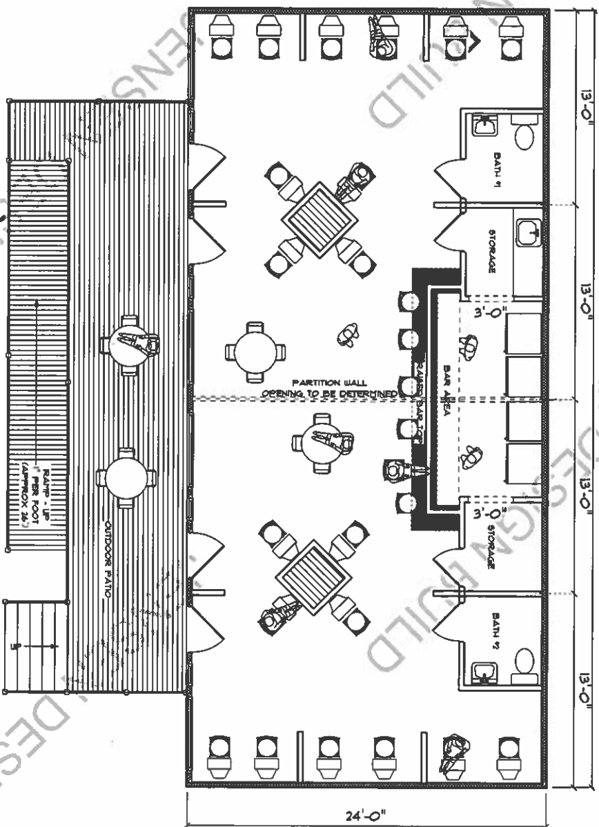
REMODELED FLOORPLAN
