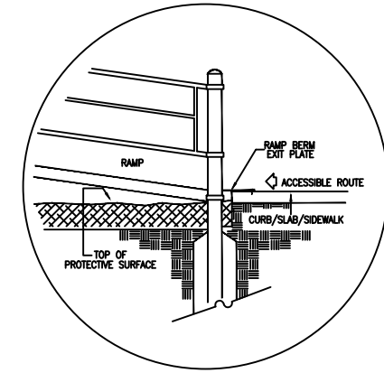
SUGGESTED RAMP BERM EXIT PLATE 8\"/12\"/16\" DECK TO GRADE/DB INSTALLATION REFER TO RAMP BERM EXIT PLATE INSTALLATION SHEET
